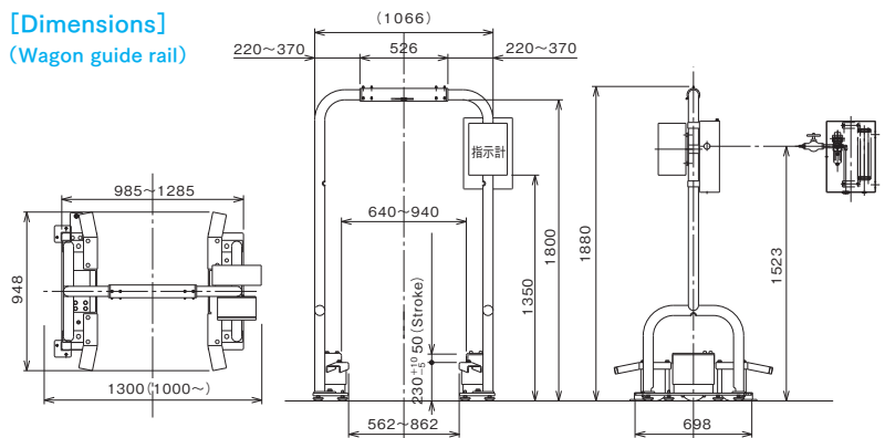
KUBOTA weight display (FC-W)
